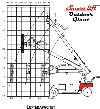
Smartlift 780
