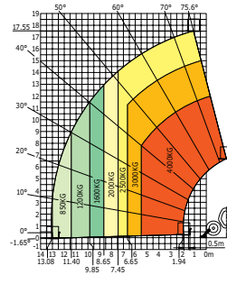
Manitou 1840
