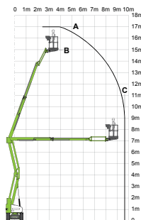
Nifty Lift HR17NE
