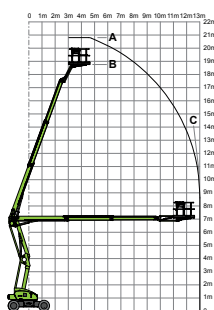
Nifty Lift HR21NE
