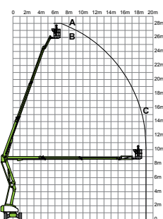
Nifty Lift HR28NE
