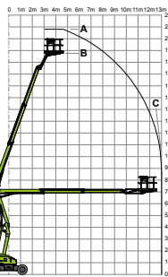
Nifty Lift HR21NE
