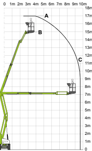
Nifty Lift HR17NE
